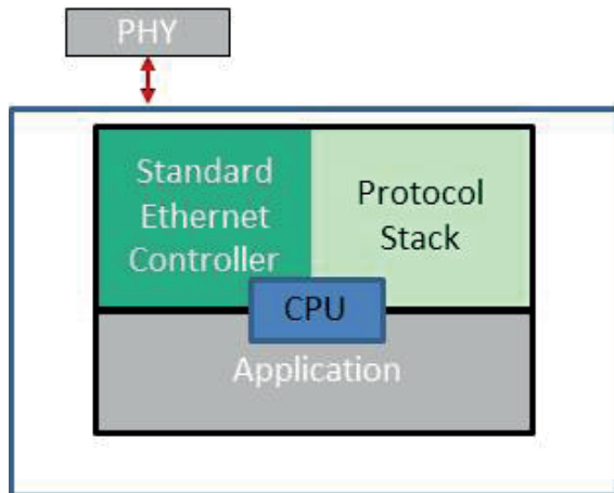
Fig. 28: Field device with software solution
