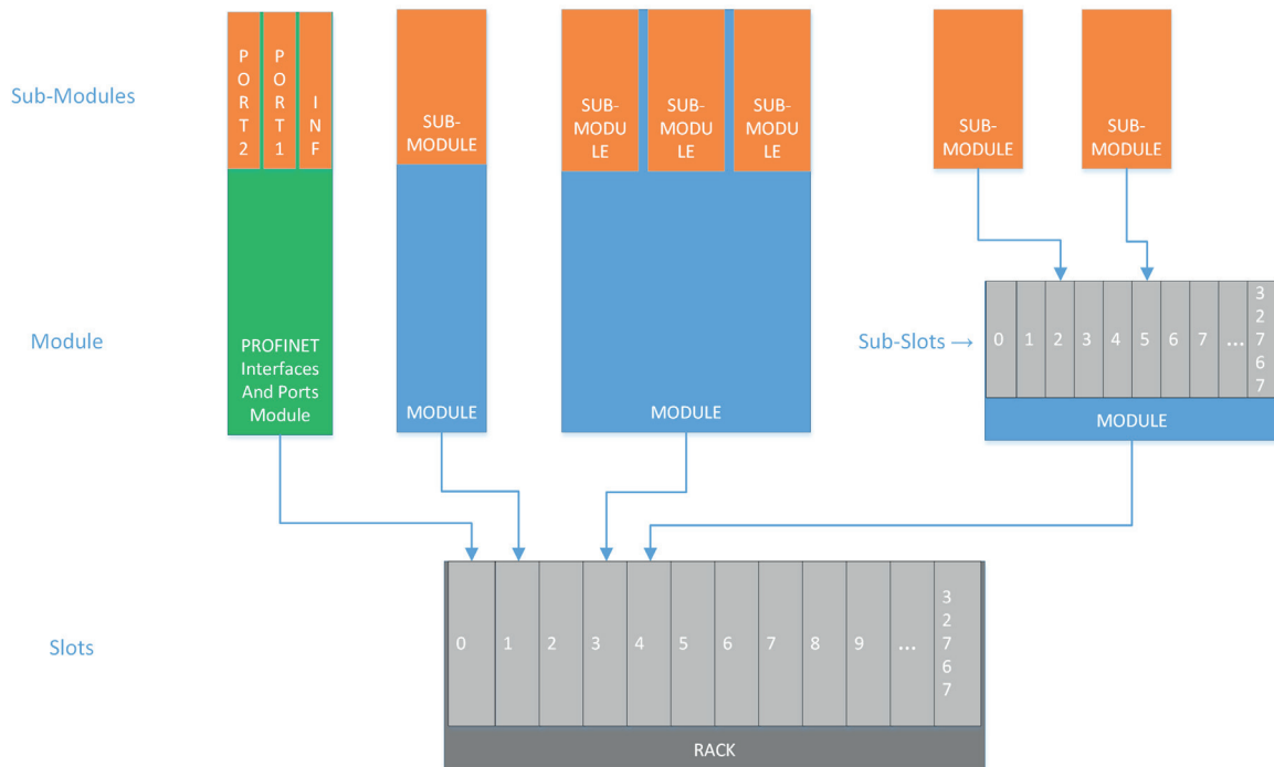
Fig. 3: Device model of a PROFINET field device
