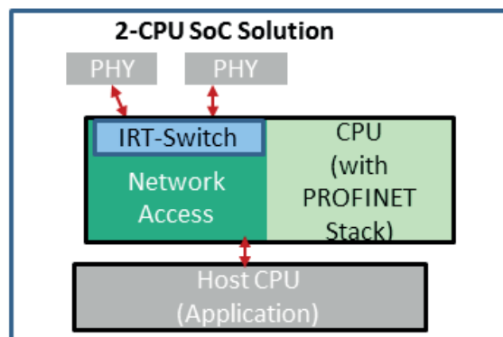
Fig. 31: Field device with host CPU and ASIC (SoC), PROFINET stack on ASIC CPU, and application on host CPU
