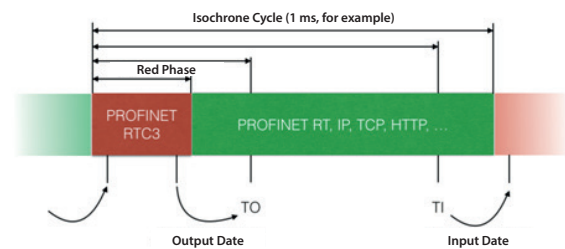
Fig. 5: Schematic representation of an isochronous cycle
