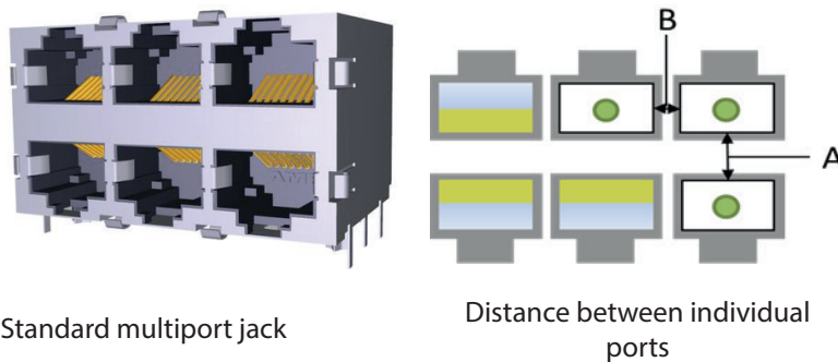
Fig. 14: Multiport device
