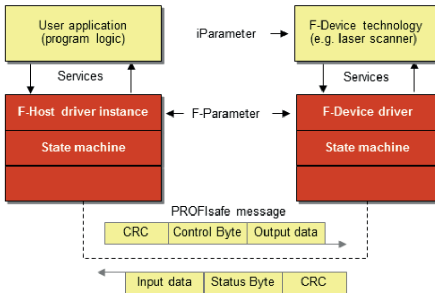
Fig. 23: PROFIsafe-layers in F-host and F-device
