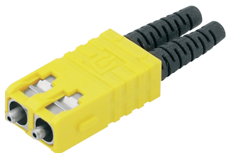
SCRJ plug connector in IP20
