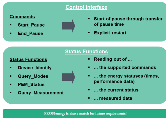
Fig. 26: PROFlenergy commands
