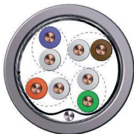
Fig. 7: Cross-section through an 8-wire PROFINET cable
