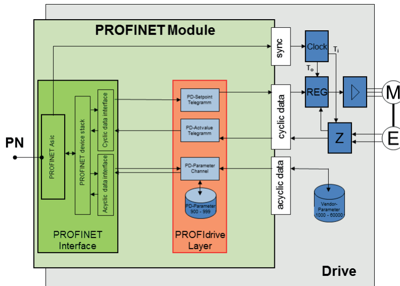
Fig. 25: PROFdrive interface
