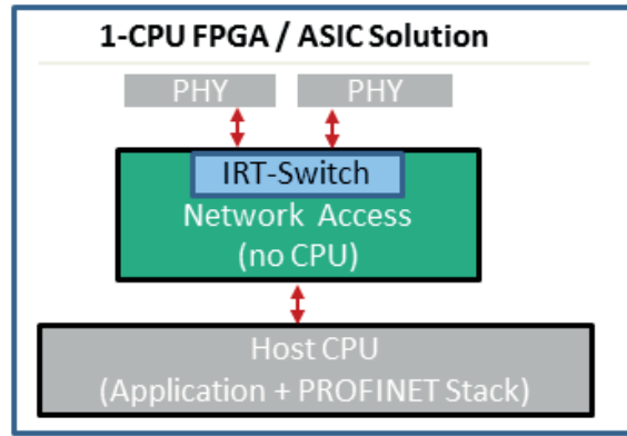
Fig. 29: Field device with host CPU and simple ASIC/FPGA, application, and PROFINET stack on host CPU
