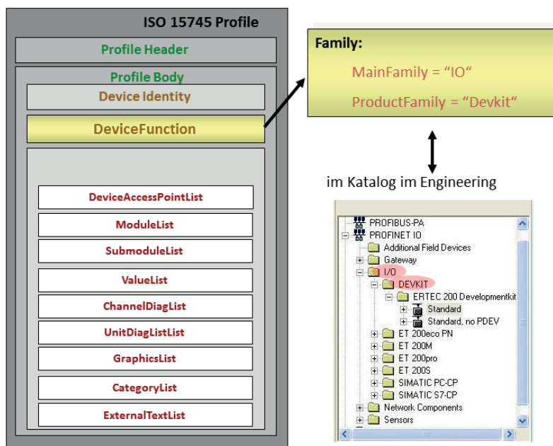
Fig. 19: Interaction between GSD and engineering
