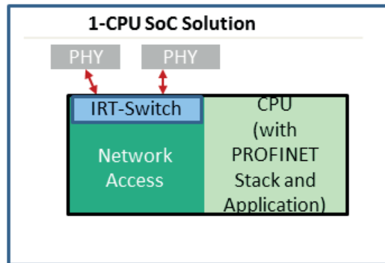
Fig. 30: Field device without host CPU with ASIC (SoC), application, and PROFINET stack on ASIC CPU
