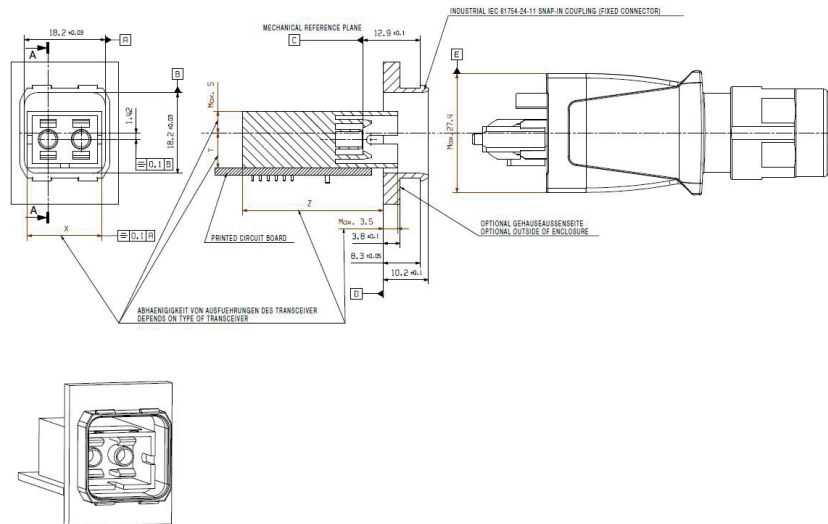
Fig. 13: Design rules for SCRJ Push-Pull connector type
