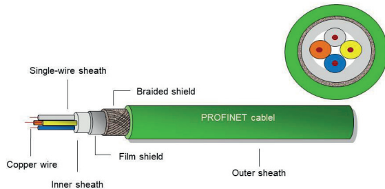
Fig. 16: 4-core PROFINET cable
