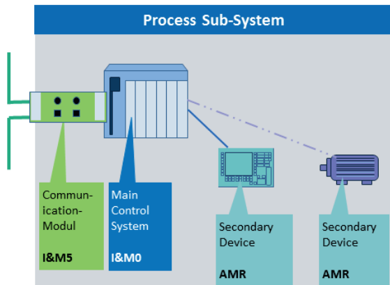
Fig. 4: Roles of the I&M and AMR data
