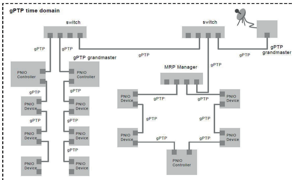
Fig. 6: Time-of-day segment synchronized via gPTP
