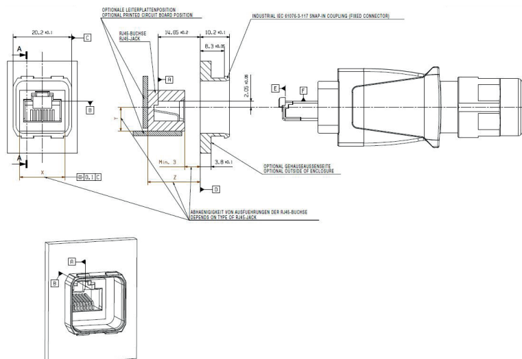
Fig. 12: Design rules for RJ45 Push-Pull connector type
