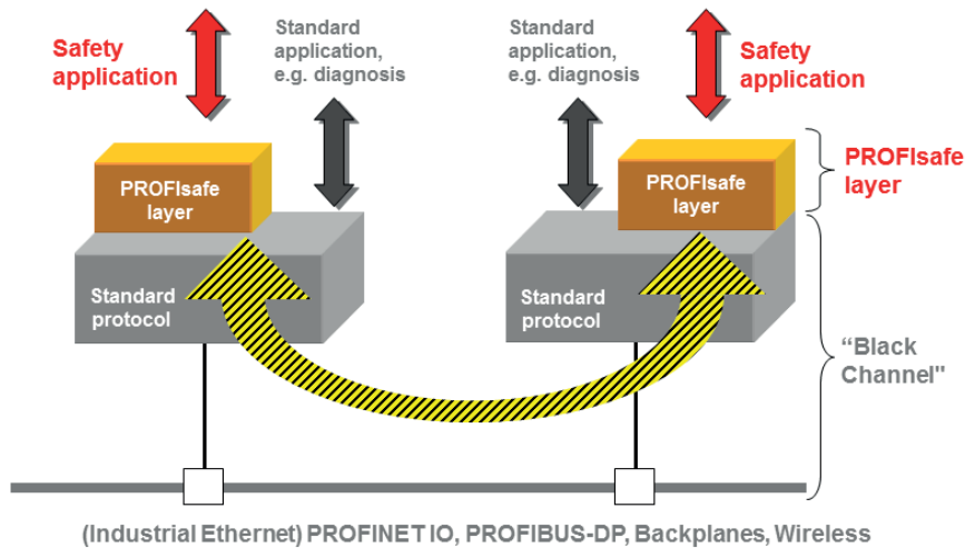
Fig. 22: "Black Channel" principle
