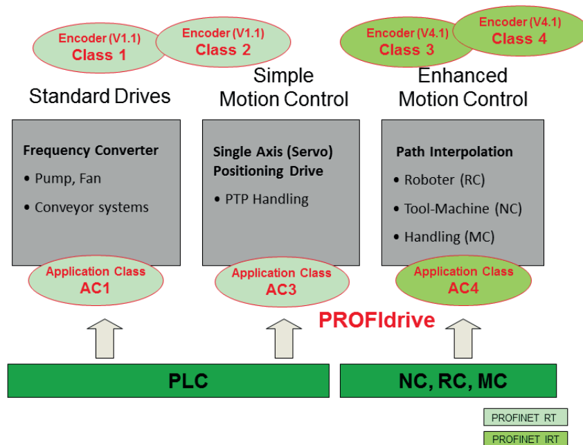
Fig. 24: PROFIdrive and Encoder application classes
